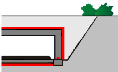
Offene Bauweise Cut and cover technique
